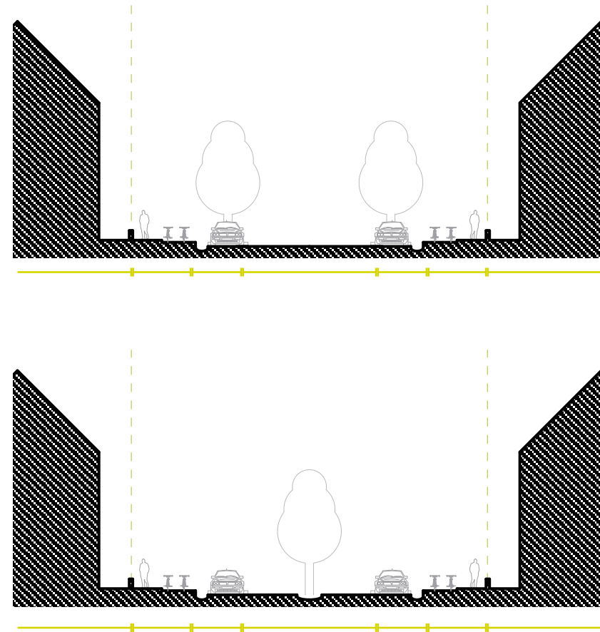
Figure 3.34 Green Boulevard Section Options
